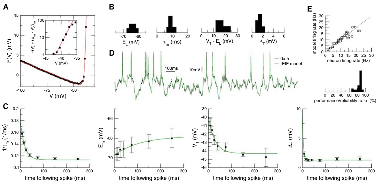
Fig. 3 GABAergic cortical interneuron models derived using the dynamic I-V methodology. a The function F(V) = -I_{\text{dyn}}(V)/C for a fast-spiking interneuron is plotted together with the EIF model fit (red). Inset: The exponential rise of the spike generating current is shown in a semi-log plot of F(V) with the leak currents subtracted. b Distribution of the EIF model parameters for a sample of 6 of the interneurons. The histograms overlap significantly with those of pyramidal cells shown in Fig. 2. c Post-spike dynamics of the EIF model parameters are fitted to an exponential model. d Comparison of the prediction of the rEIF model (green) with experimental data (black) shows close agreement in the subthreshold region and in the prediction of spike times. Summary of the performance of the rEIF model for the 6 cells investigated. Top : Prediction of the firing rate. Bottom : Histogram of the performance measure
