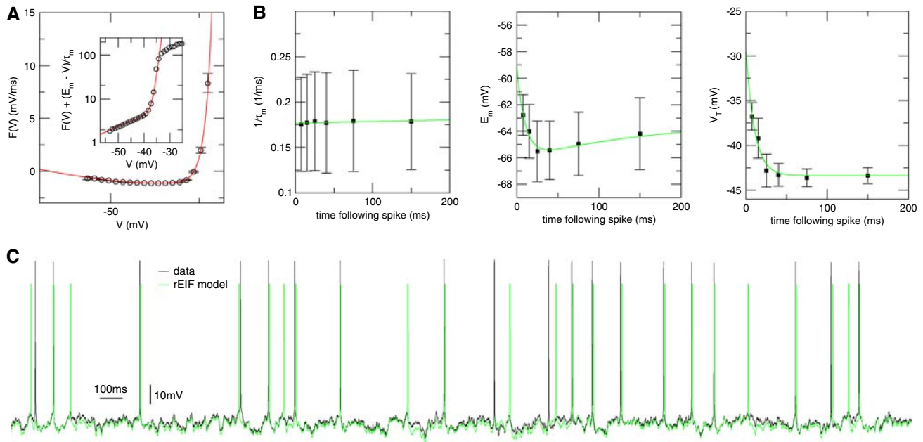
Fig. 4 Application of the dynamic I-V method with conductance injection. a The function F(V) = -I_{\text{dyn}}(V)/C is plotted (symbols) together with the fit (red) to the function (14). Inset: Two exponential components are clearly seen in a semi-log plot of F(V) + (E_m - V)/\tau_m with the leak currents subtracted. b Post-spike dynamics of the EIF model parameters (symbols) together with the fits to an exponential model. The time-dependent resting potential shows a clear biphasic response as was seen for layer-5 pyramidal neurons in the current-injection protocol. c Comparison of the prediction of the rEIF model (green) with experimental data again shows good agreement in the subthreshold region and in the prediction of spike times
