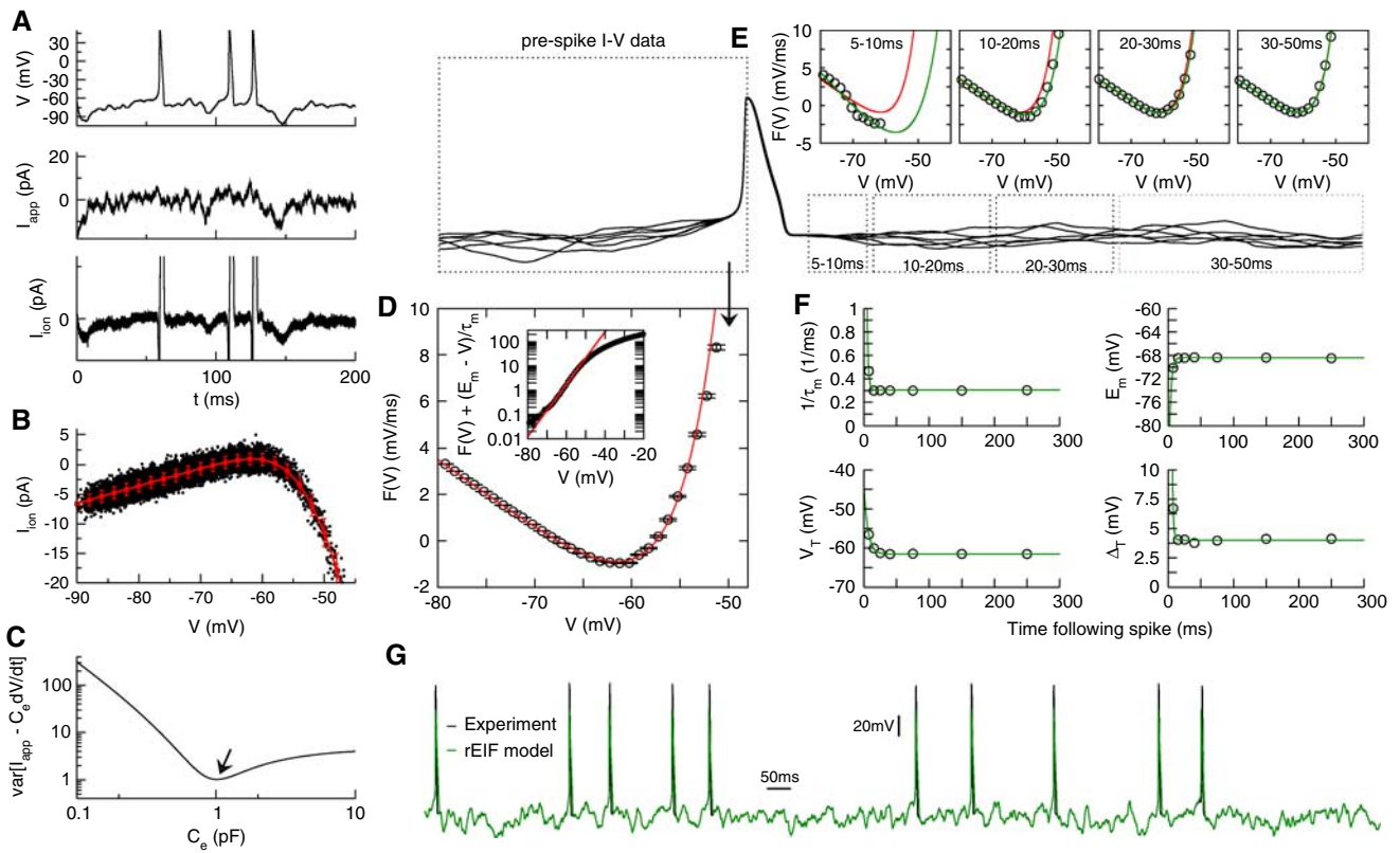
Fig. 1 Summary of the dynamic I-V curve method and its application to the Wang–Buzsáki model. The derivative of the membrane voltage (top graph), multiplied by the cellular capacitance, is subtracted from the injected current (middle graph) to yield the intrinsic membrane current I_{ion} (bottom graph). b The intrinsic membrane current I_{ion} is plotted against the membrane voltage (black symbols). The dynamic I-V curve (red symbols) is obtained by averaging I_{ion} in small voltage bins. Error bars represent the standard deviation. c Measuring the cellular capacitance. At a fixed subthreshold voltage, the dynamic membrane current I_{ion} = I_{app} - C_e dV/dt has a variance that depends on the value of C_e used in the calculation; the correct value of C_e corresponds to the point of minimal variance. d Relating dynamic I-V curves and non-linear integrate-and-fire models. The function F(V) = -I_{dyn}(V)/C_e (symbols) is plotted as a function of voltage, together with the EIF model F(V) (red line). Inset: semi-log plot of F(V) with leak current subtracted, showing a nearly exponential run-up. e Spike-triggered dynamic I-V curves. The functions F(V) measured in small time slices after each spike (symbols) are plotted together with the EIF F(V) (green) and the pre-spike I-V curve as a reference (black). At early times it is clearly seen that both the conductance and the spike threshold are significantly increased. f Dynamics of the EIF model parameters during the refractory period. The parameters obtained from the fits of the I-V curves (symbols) are plotted as a function of the time since the last spike (black) and fitted with exponential functions (green). g Comparison of the prediction of the refractory EIF (rEIF) model (green) with a voltage trace of the Wang–Buzsáki model (black) shows excellent agreement, with 96% of the spikes correctly predicted by the EIF model within a 5 ms window
