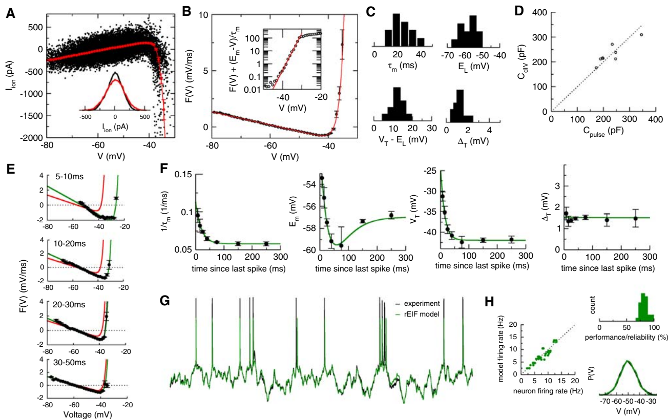
Fig. 2 Application of the dynamic dV method to layer-5 pyramidal cells. a The intrinsic membrane current is plotted against the membrane voltage ( I_{ion} vs V , black symbols). The dynamic dV curve (red) is clearly seen to comprise a linear component in the subthreshold region followed by a sharp activation in the region of spike initiation. Inset: Examination of the variance of I_{ion} near the resting potential in the absence (black) or presence (red) of injected current suggest that the majority of the variance comes from intrinsic noise. The function F(V) = -I_{dyn}(V)/C is plotted here (symbols) together with the EIF model fit (red). Inset: The exponential rise of the spike generating current is shown in a semi-log plot of F(V) with the leak currents subtracted. c Histograms of the EIF model parameters for a sample of ( N = 12 ) of pyramidal cells, showing considerable heterogeneity in the response properties of neurons in this population. d The cellular capacitance calculated with our optimization method (see text) is compared to the result of the standard current-pulse protocol, showing good agreement between the two methods. e Spike-triggered dynamic dV curves measured in small time slices after a spike are plotted together with the EIF model (green) and the pre-spike dV curve (red). f Post-spike dynamics of the EIF model parameters (symbols) together with the fits to an exponential model. While conductance and spike threshold could be accurately fitted with a single exponential, the variation in the equilibrium potential required two exponential components for a good fit. The spike width did not vary significantly for these cells. g Comparison of the prediction of the rEIF model (green) with experimental data shows good agreement in the subthreshold region and in the prediction of spike times. h Summary of the performance of the rEIF model for the 12 cells investigated. Left: Prediction of the firing rate. Top right: Histogram of the performance/reliability (%). Bottom right: Voltage distribution for the rEIF model (green) compared to the experimental data (black). The figure is adapted from Adelman et al. 2008
